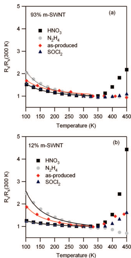
Figure 3. Normalized R_s as a function of temperature for (a) 93% metallic SWNT film and (b) 12% metallic SWNT film as-produced and after treatment in HNO 3 , N 2 H 4 , and SOCl 2 .
